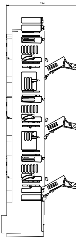
OPEN POSITION
