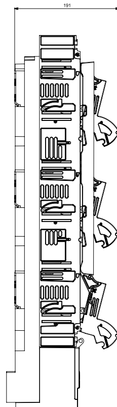
PARKING POSITION
