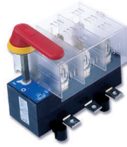
RAB2P3/OHY + fuse link shroud
