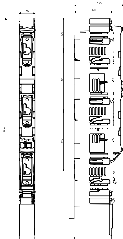
CLOSED POSITION
