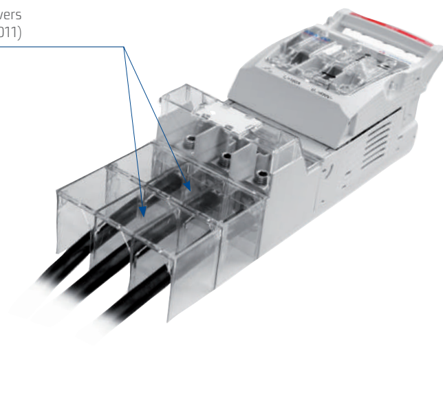
RBK 00 pro-V120 with V-clamp for connection of sector-shaped conductors with cross-section up to 120 mm 2
