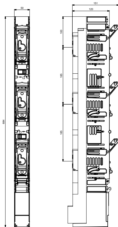
CLOSED POSITION
