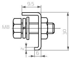
Clamp 16-120 mm 2 Klemme 16 – 120 mm 2
