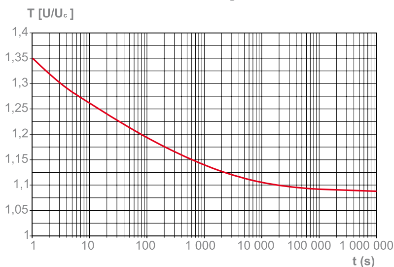
Diagram no. 2. typical characteristics of temporary overvoltages T withstand curve
