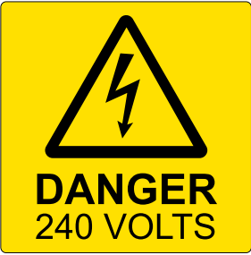
SL5050D240
